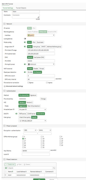
Fig. 3 - 4.3 Fase 1 "ravpn": Dialup en port1, Mode Connection y split tunnel a 10.0.11.0.
