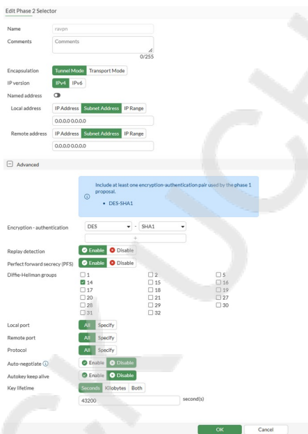
Fig. 4 - 4.4 Fase 2: Tunnel Mode, 0.0.0.0/0, PFS (DH 14), Replay detection, 43200 s.
